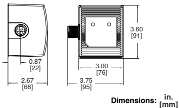
Figure 4: Dimensions
