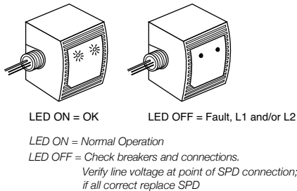
Figure 3: Diagnostic Operation
