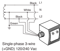
Figure 2: Wiring Diagrams
