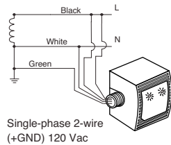
Figure 3: Diagnostic Operation
